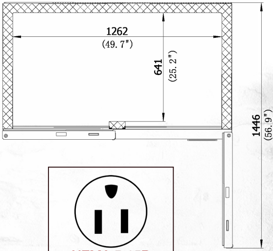
PRODUCT DRAWINGS
